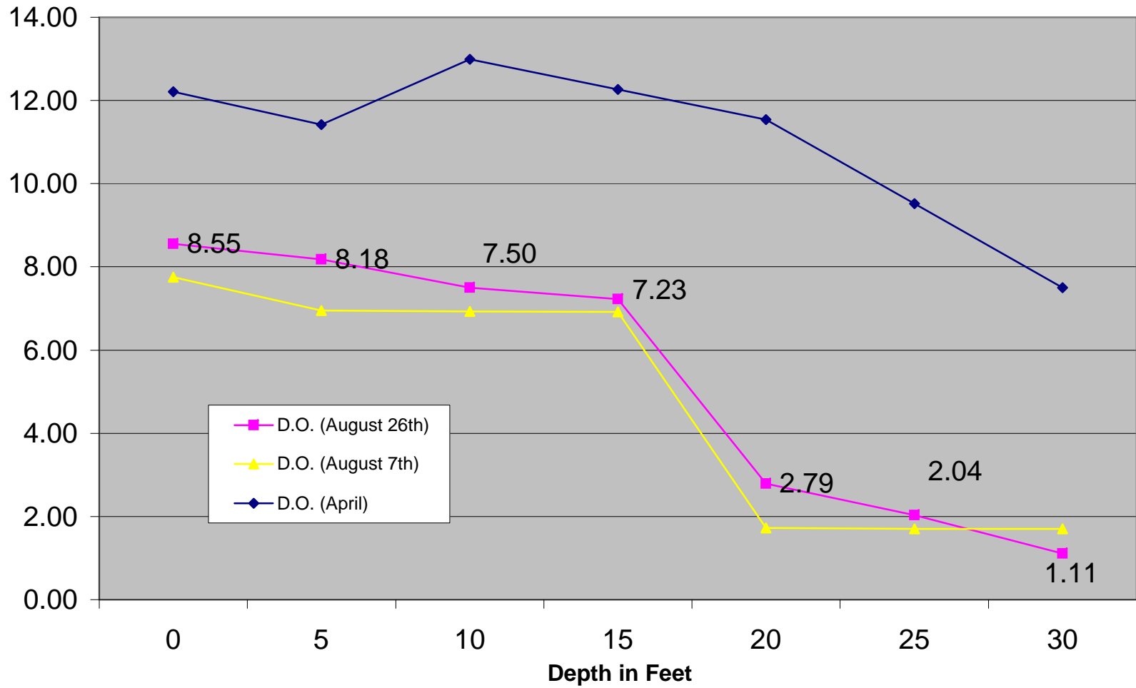
Dissolved Oxygen vs. Depth (April vs. August)
